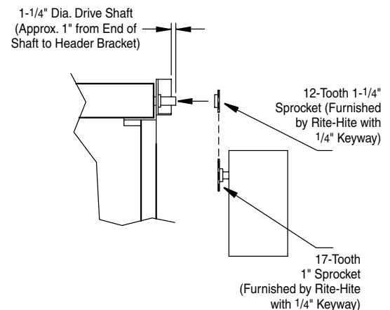
Operator Ready 8010 Dok-Dor Operated by Others Mounting Details
